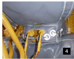
PHOTOS 1-4 Cat D11T manifold, turbo, e/pipe and muffler blankets PHOTOS 5-7 Cat 815K manifold, turbo and e/pipe blankets
